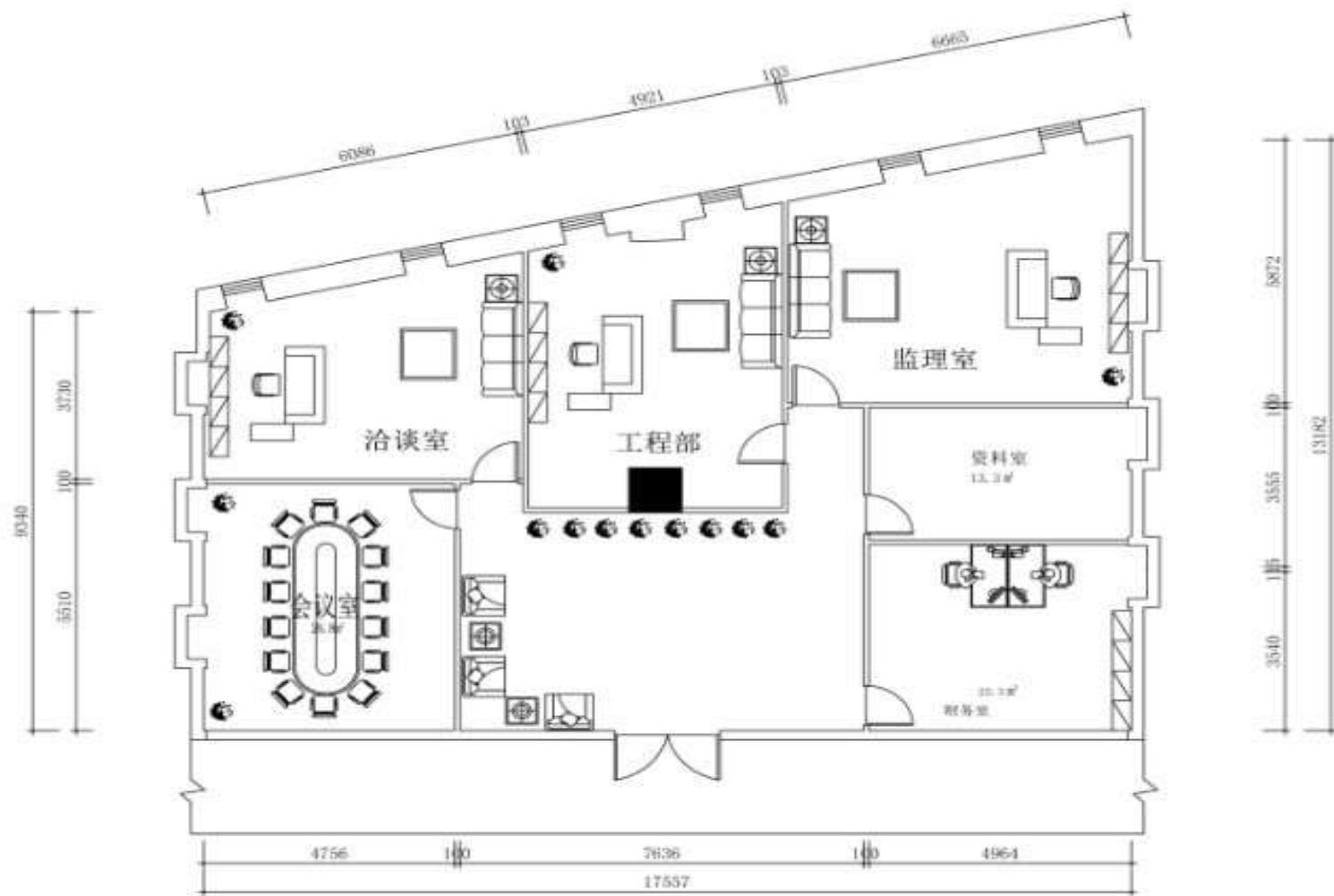
PLANE ANALYSIS DIAGRAM / 平面图
